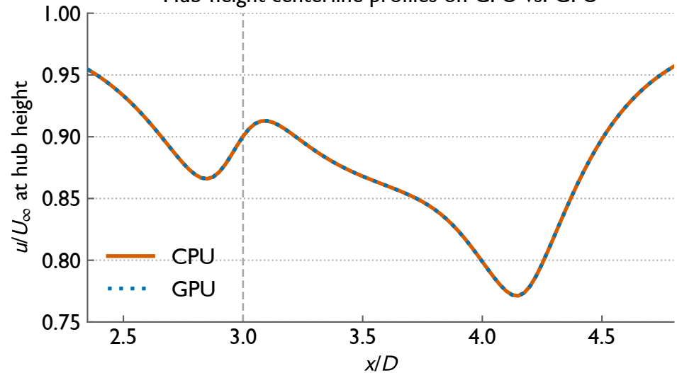
Hub-height centerline profiles on CPU vs. GPU
