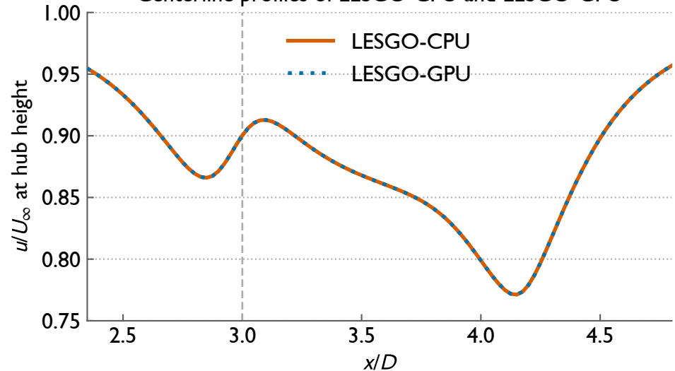
Centerline profiles of LESGO-CPU and LESGO-GPU
