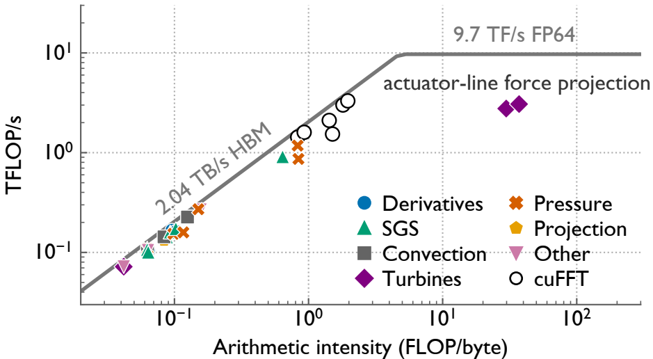
Roofline plot for LESGO kernels on AI00 GPUs
