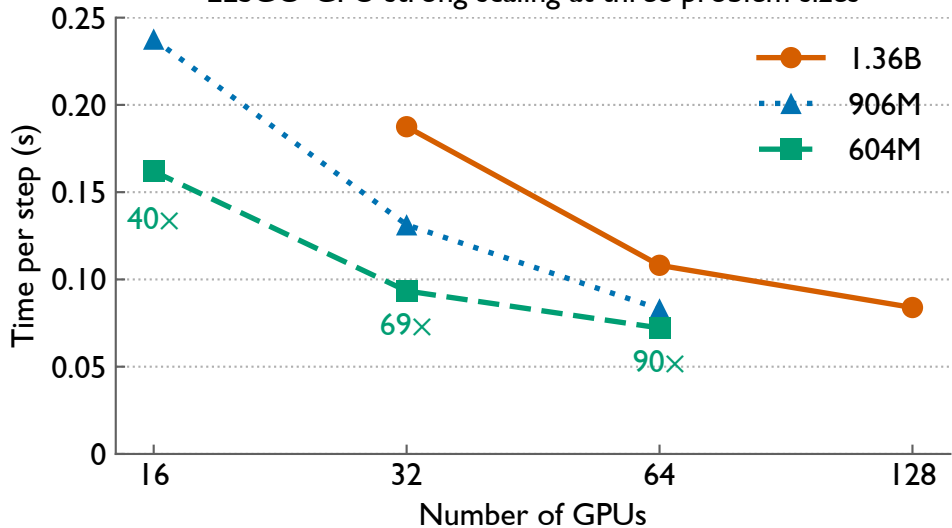
LESGO-GPU strong scaling at three problem sizes
