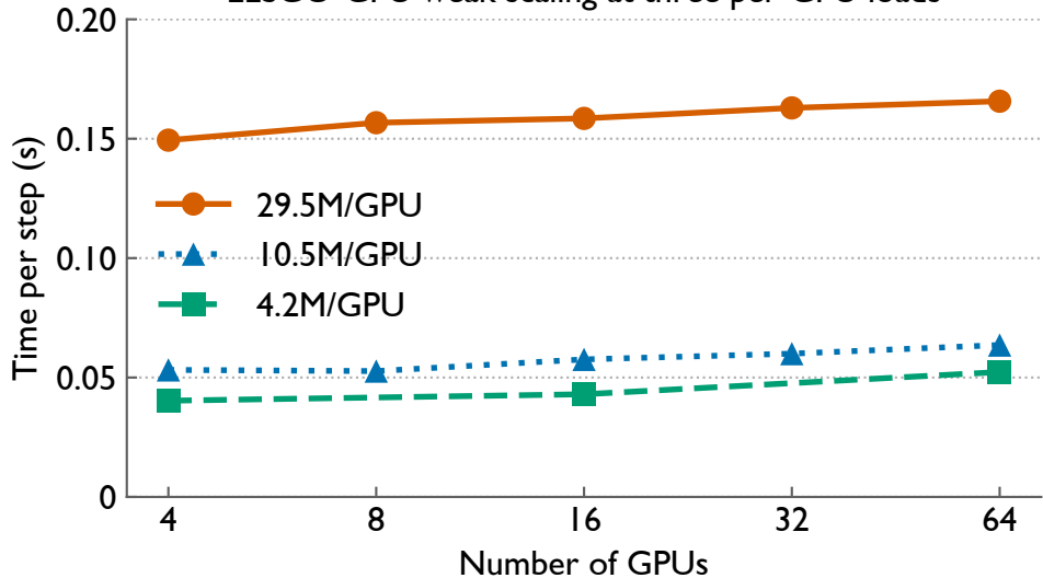
LESGO-GPU weak scaling at three per-GPU loads
