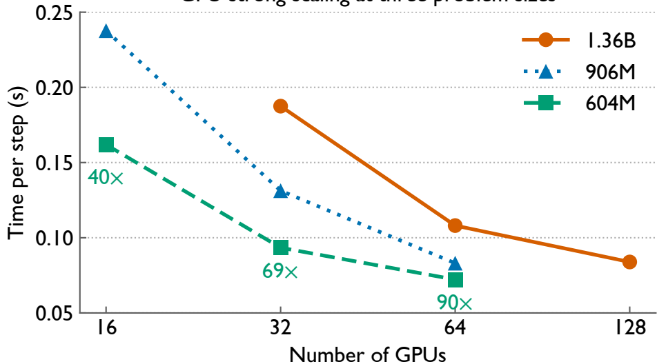
GPU strong scaling at three problem sizes
