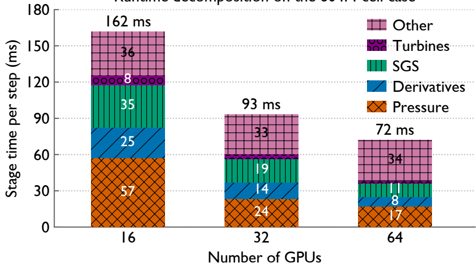
Runtime decomposition on the 604M-cell case
