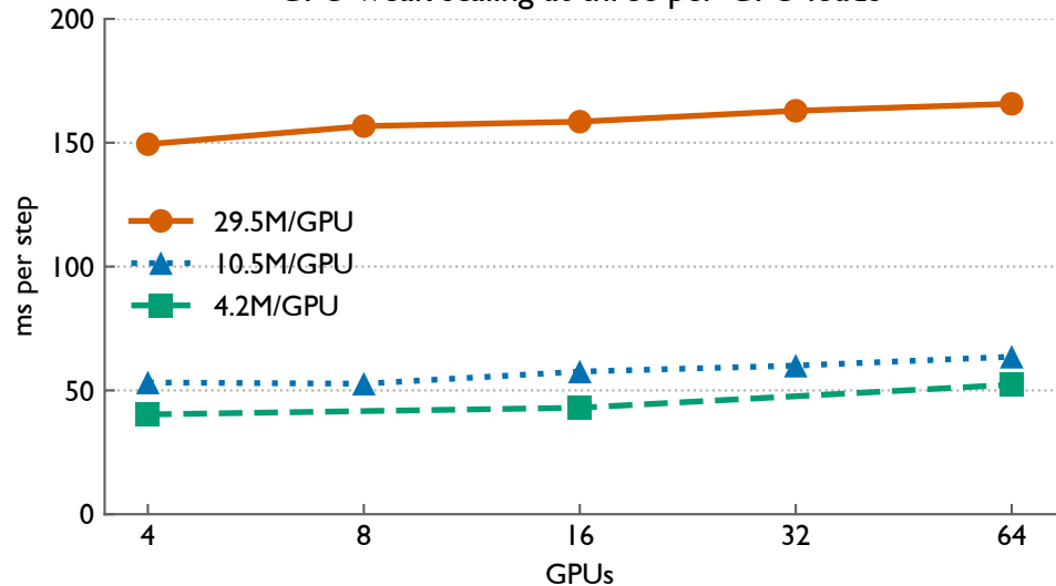
GPU weak scaling at three per-GPU loads
