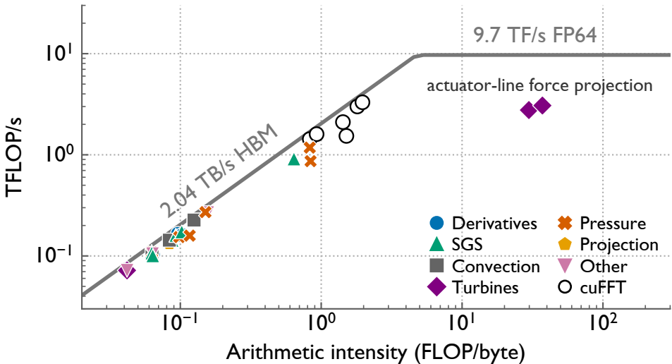
Roofline plot for LESGO kernels on A100 GPUs
