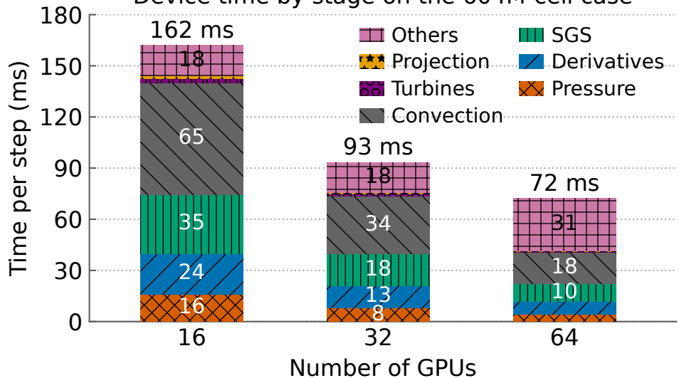
Device time by stage on the 604M-cell case
