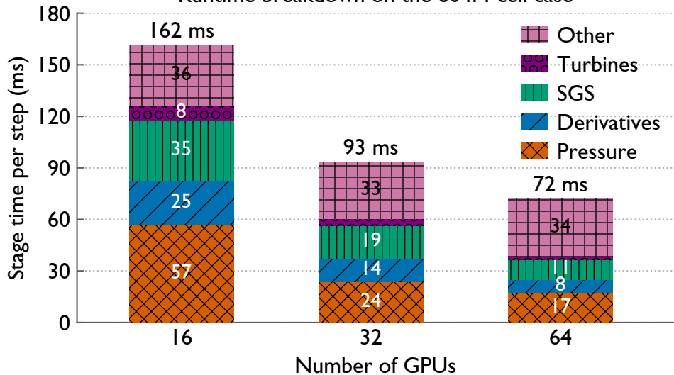
Runtime breakdown on the 604M-cell case
