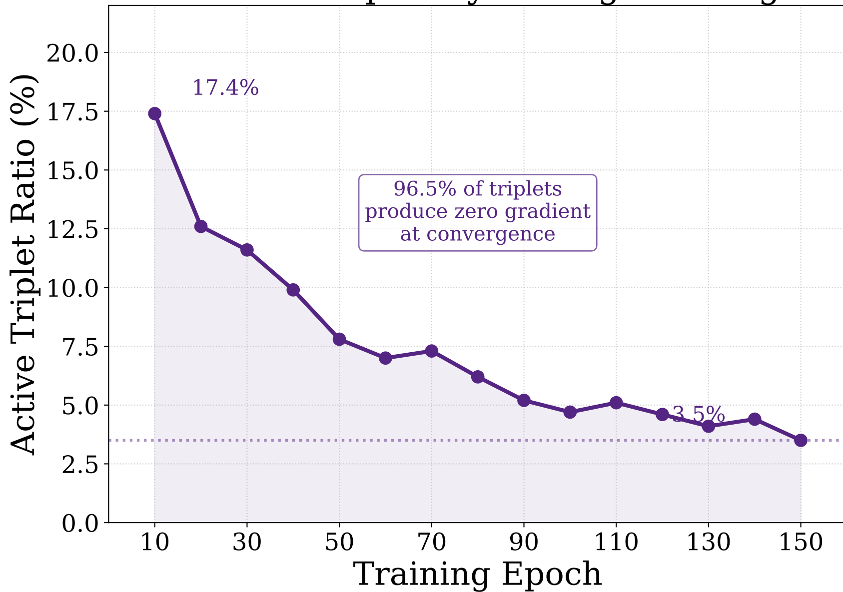
Gradient Sparsity During Training
