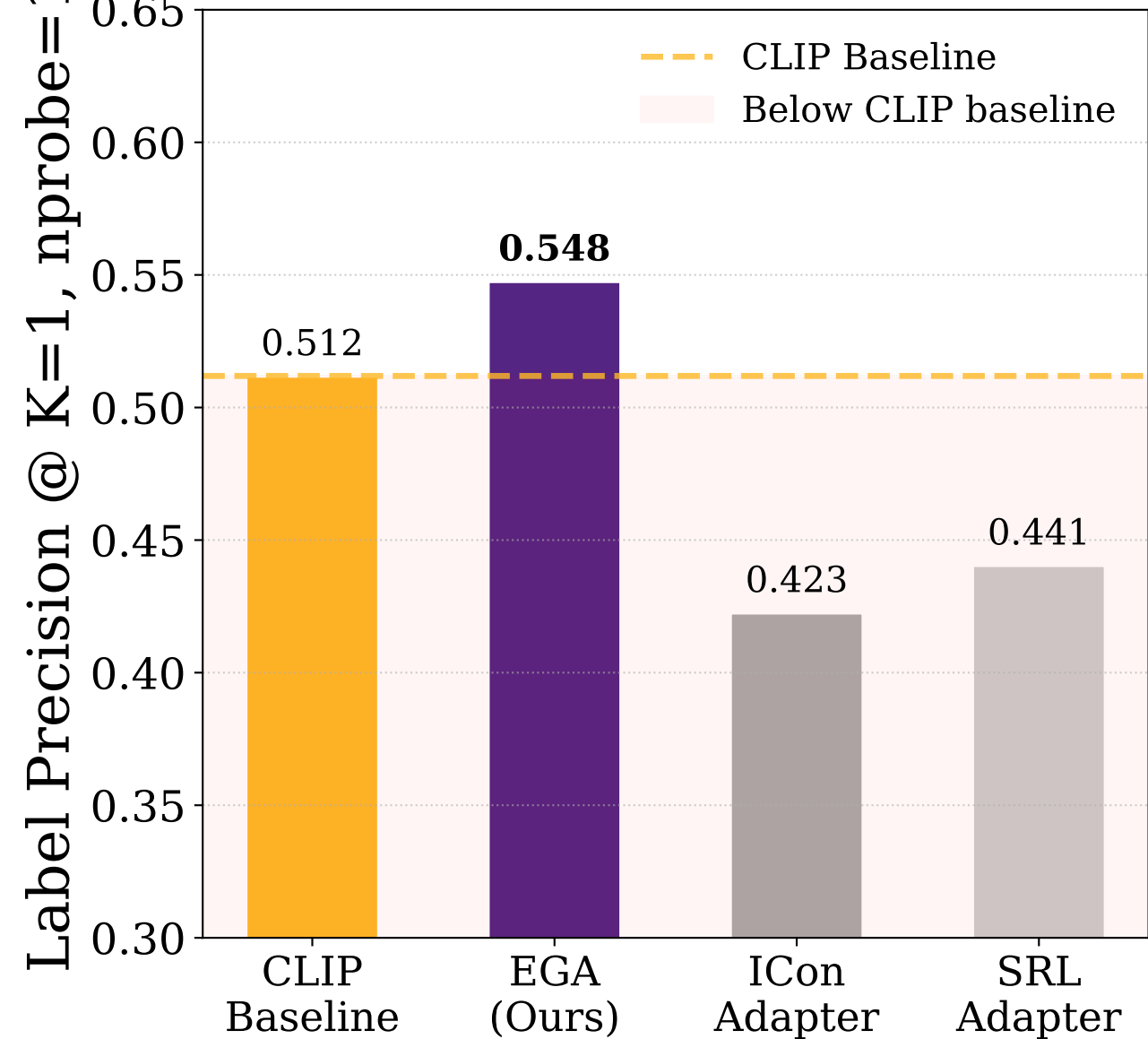
OOD Retrieval on Unseen Classes
