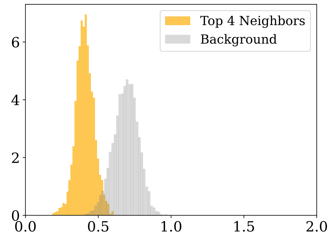
Latent Manifold ( K = 4 )
