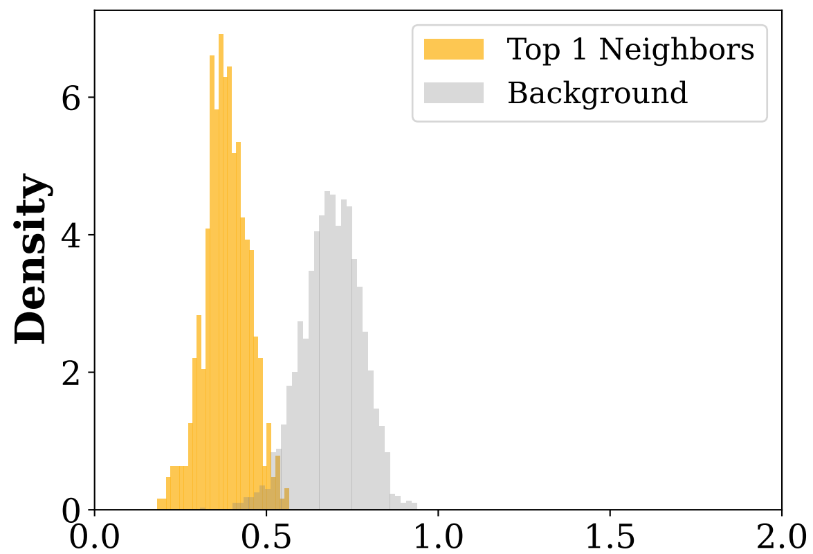
Latent Manifold ( K = 1 )
