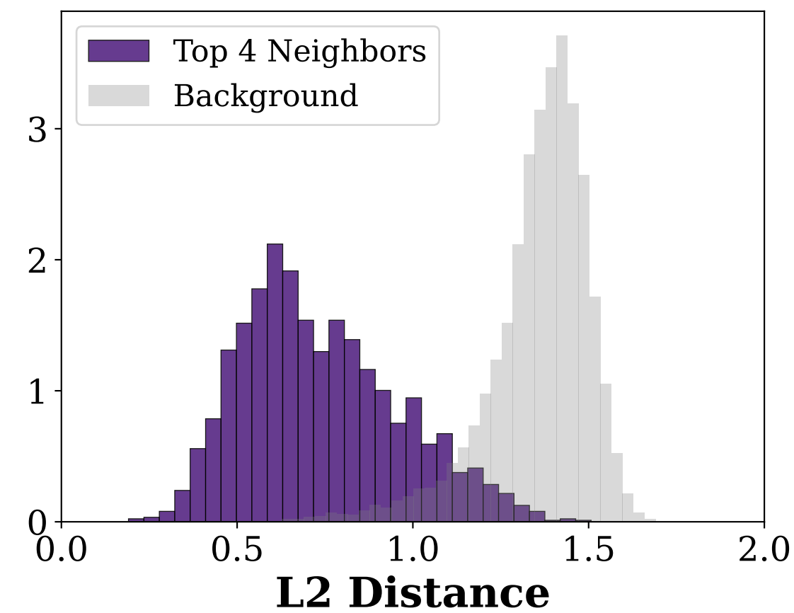
EGA Flattened Space ( K = 4 )
