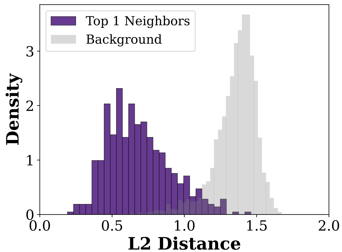
EGA Flattened Space ( K = 1 )
