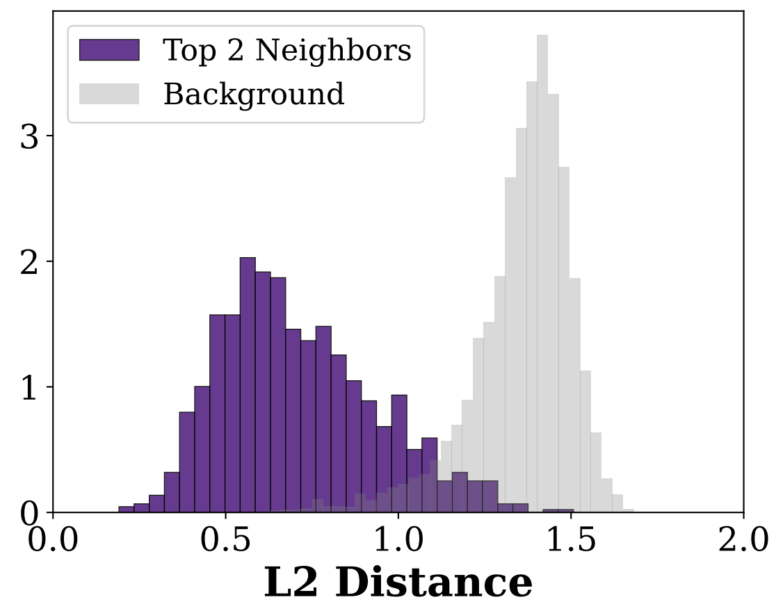
EGA Flattened Space ( K = 2 )
