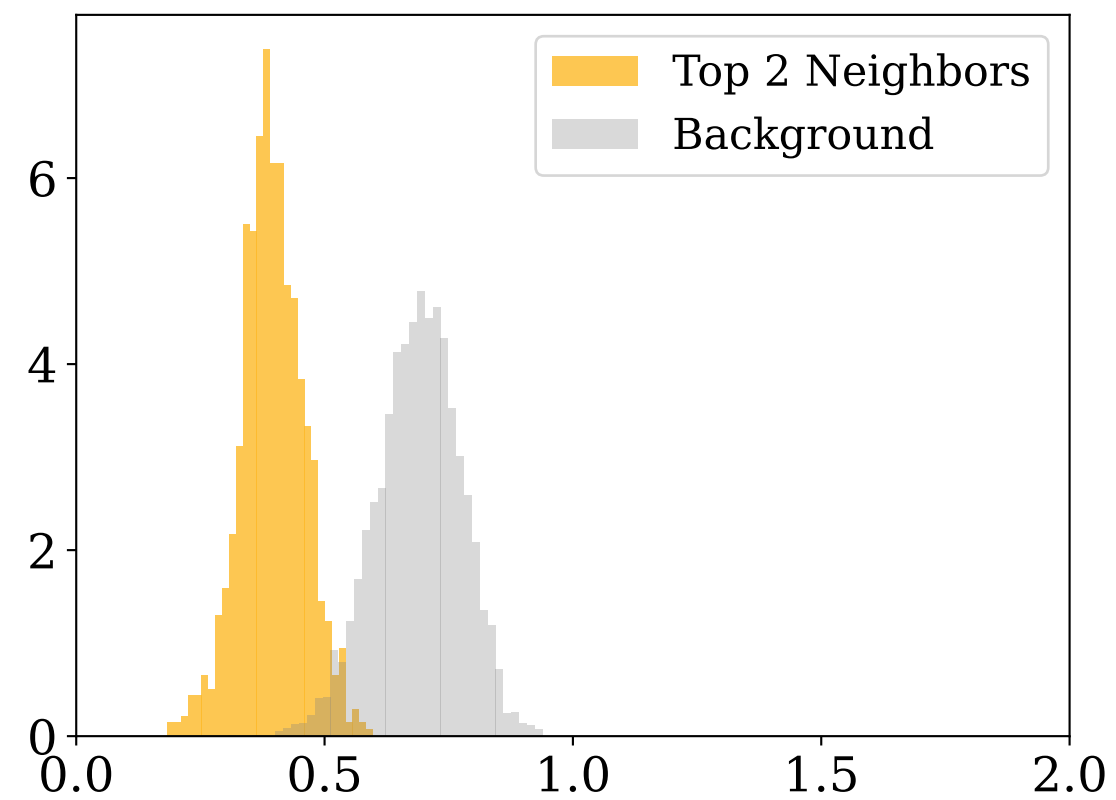
Latent Manifold ( K = 2 )
