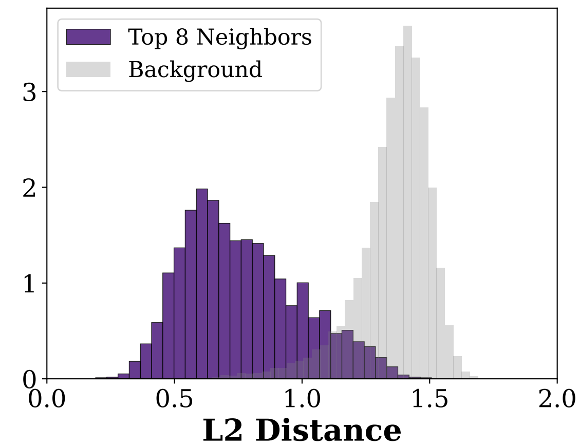
EGA Flattened Space ( K = 8 )
