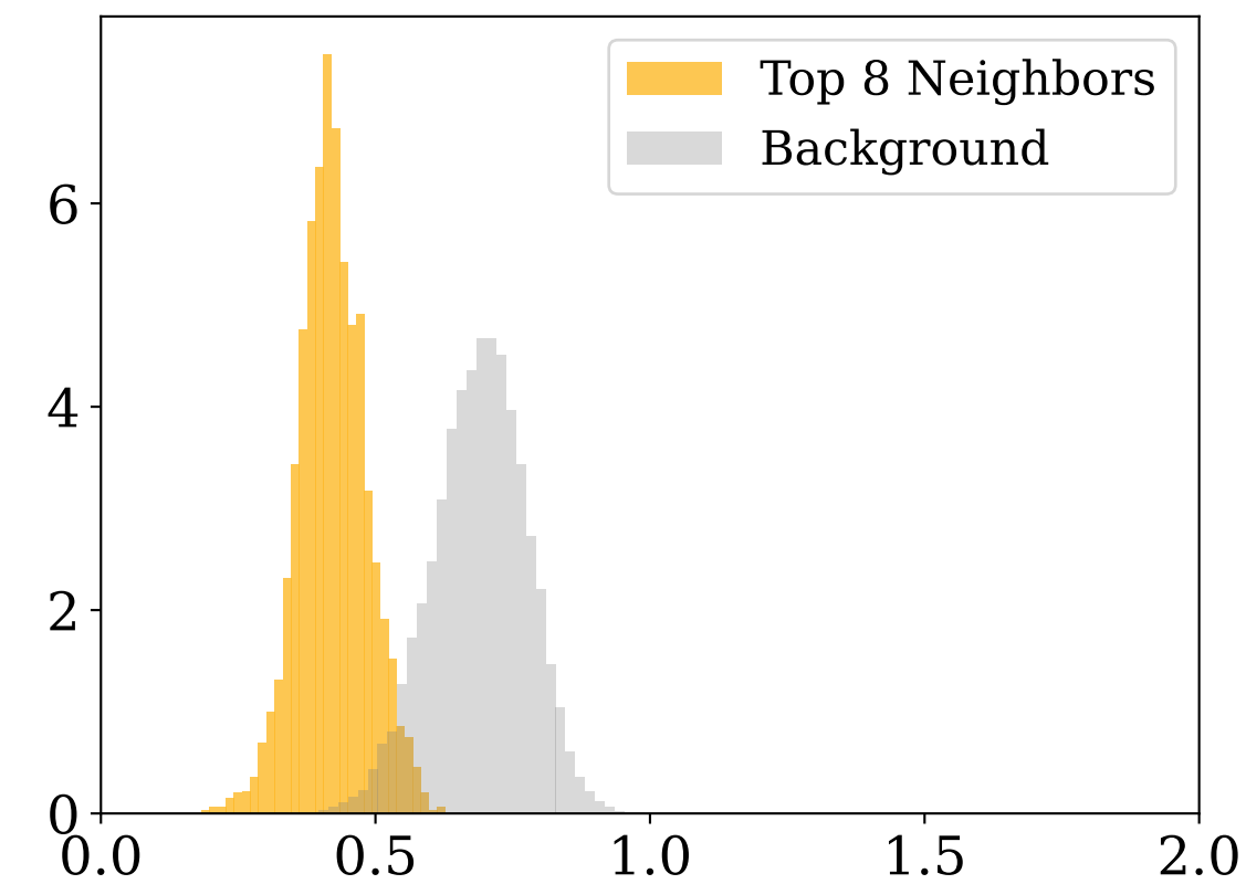
Latent Manifold ( K = 8 )
