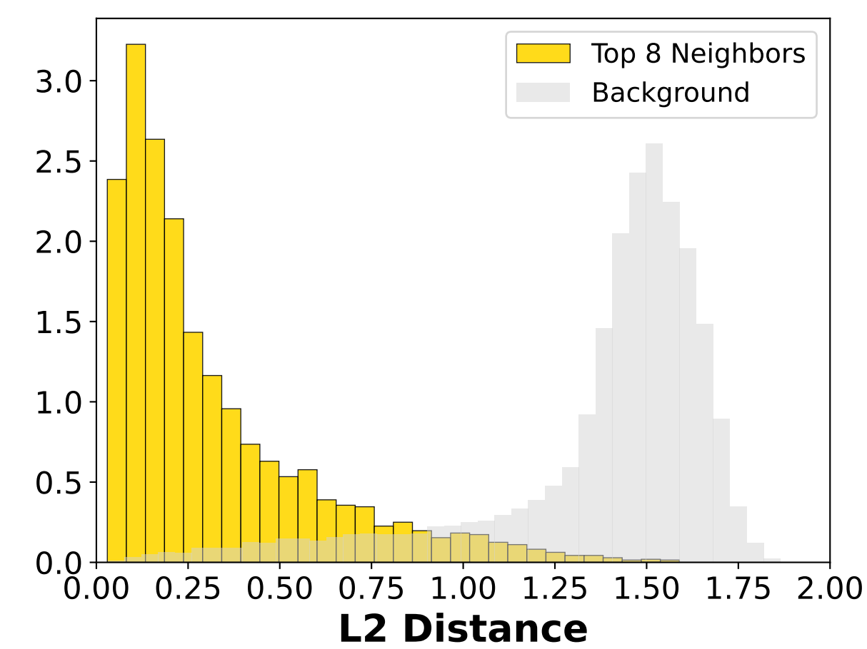
EGA Flattened Space (K=8)
