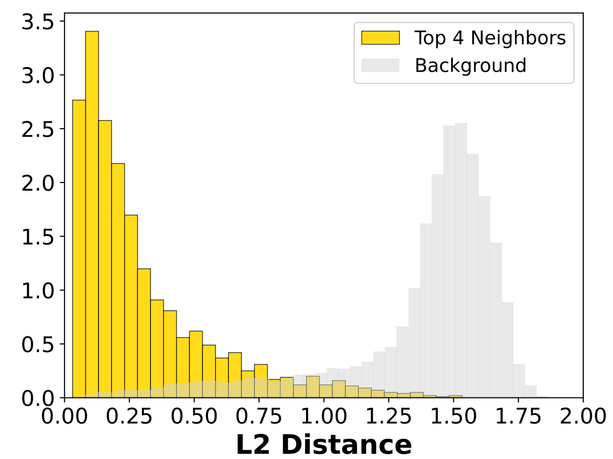
EGA Flattened Space (K=4)
