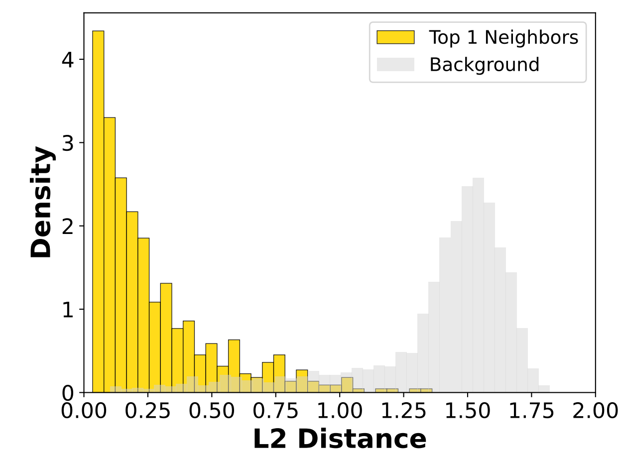
EGA Flattened Space (K=1)
