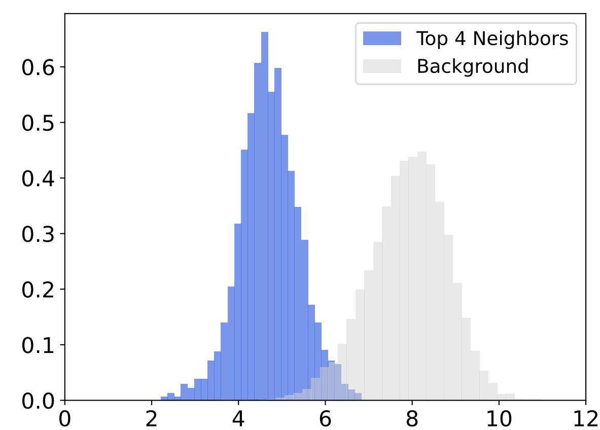
CLIP Latent Manifold (K=4)
