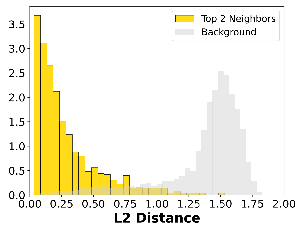
EGA Flattened Space (K=2)
