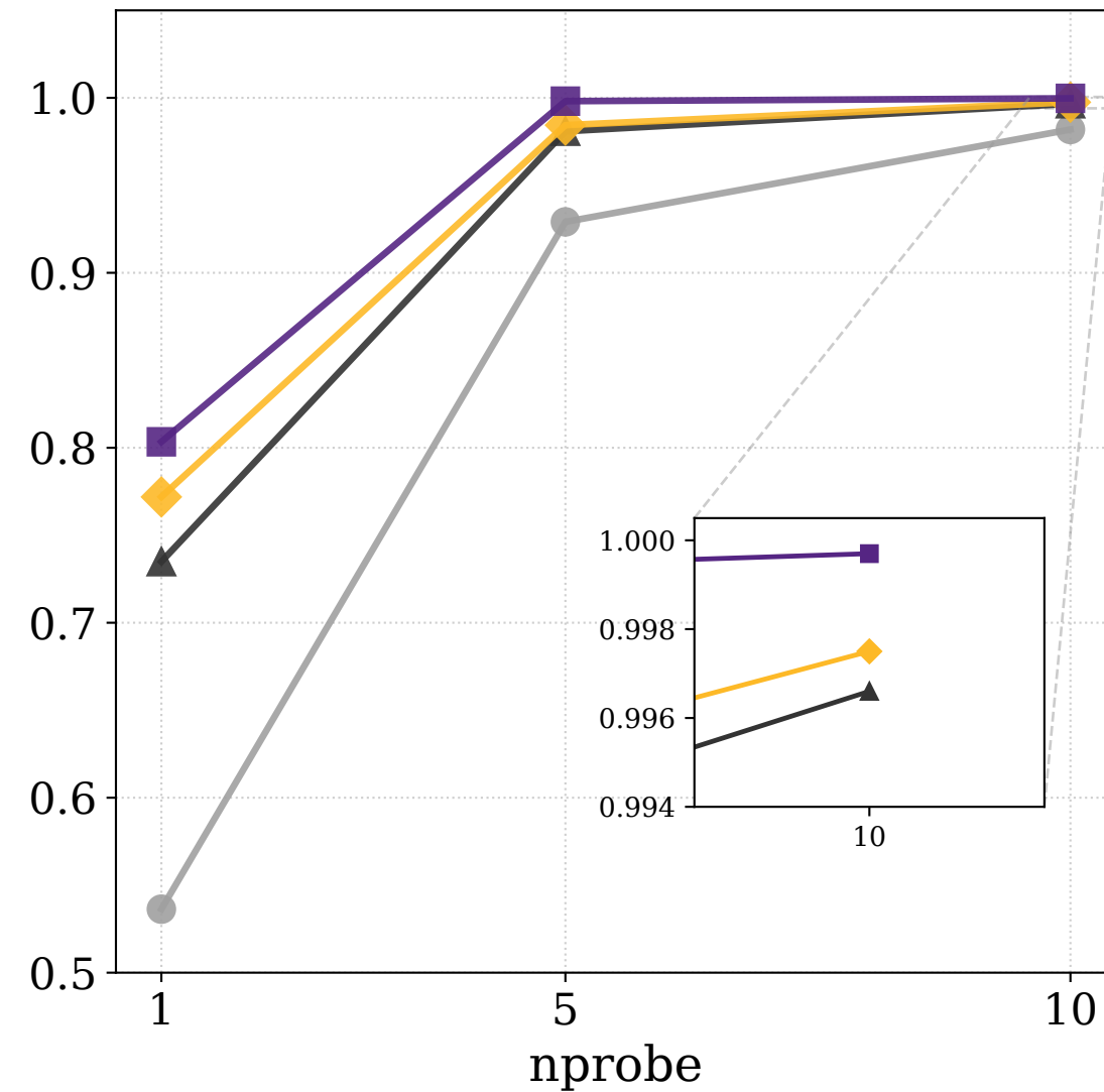
Recall@10
