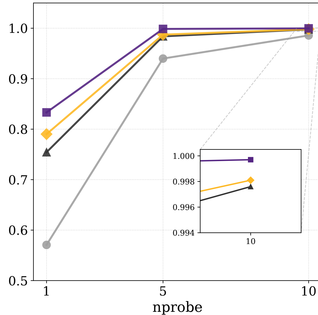
Recall@5
