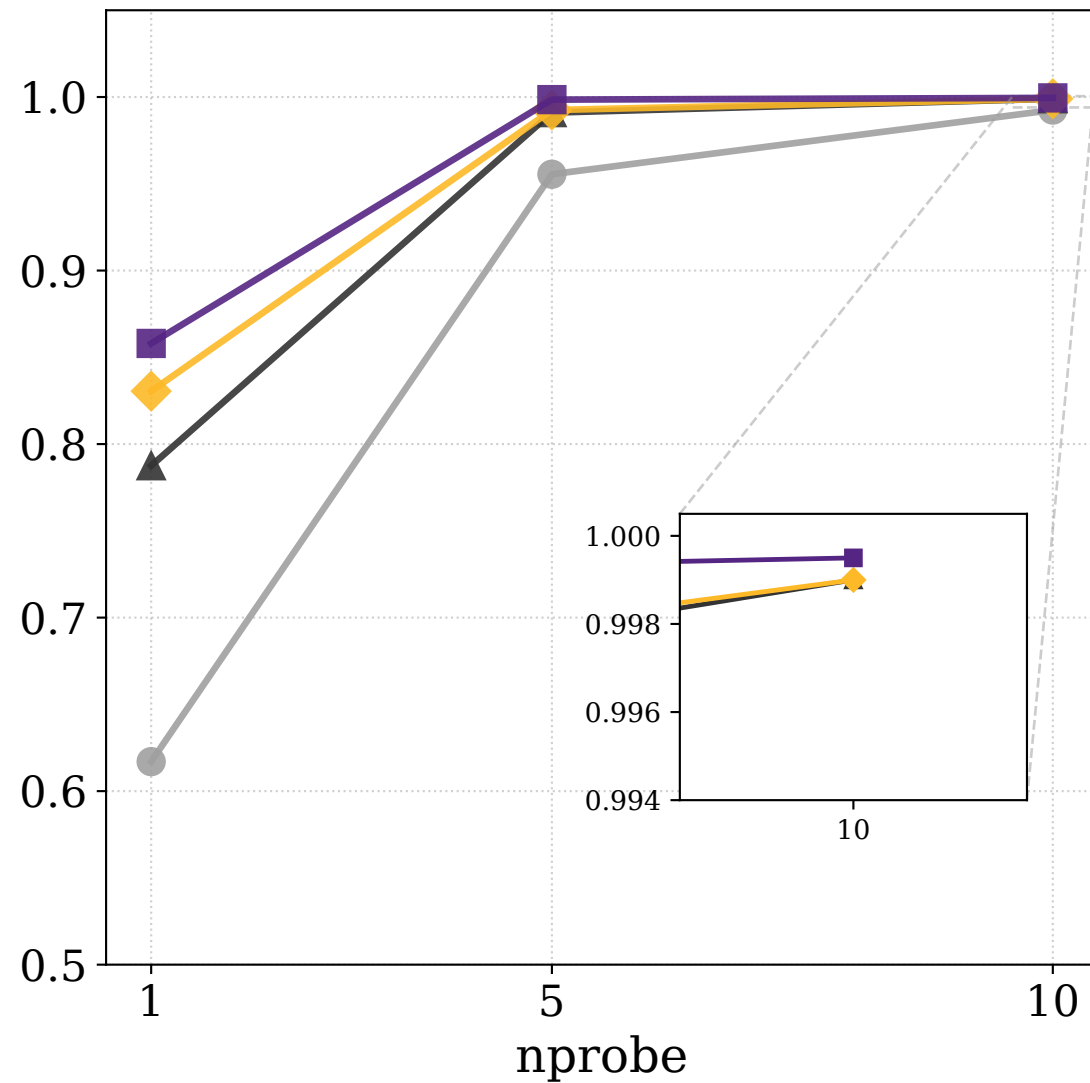
Recall@1
