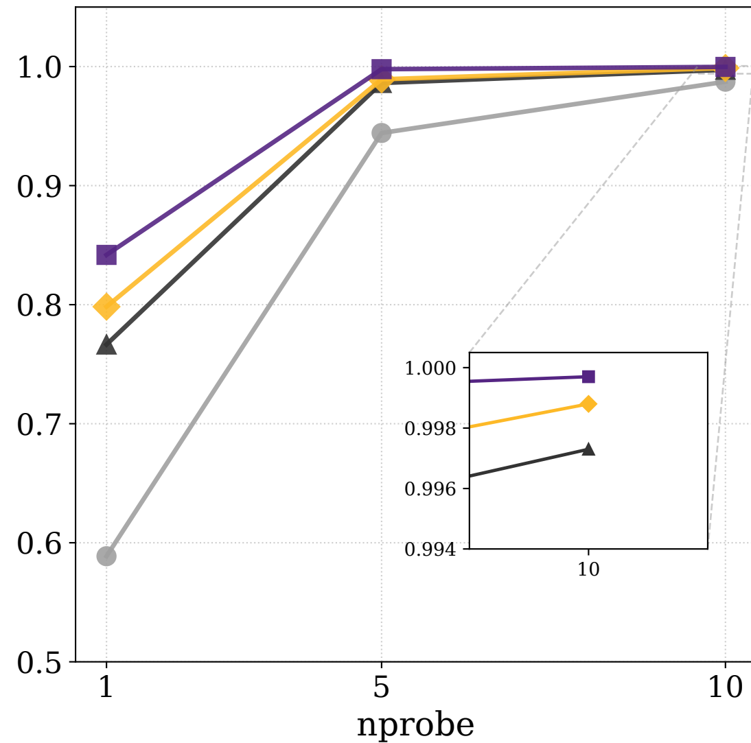
Recall@3
