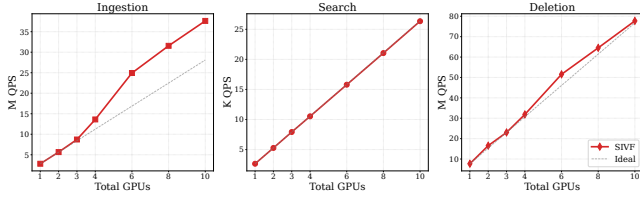
Figure 12: Scalability of SIVF core operations across a three node cluster with up to 10 GPUs.
