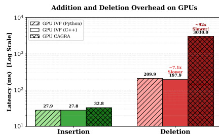
Figure 1: The asymmetry between insertion and deletion. [Dongfang: Add a result of tombstone deletion: memory footprint vs. number of deletions for streaming vectors]
