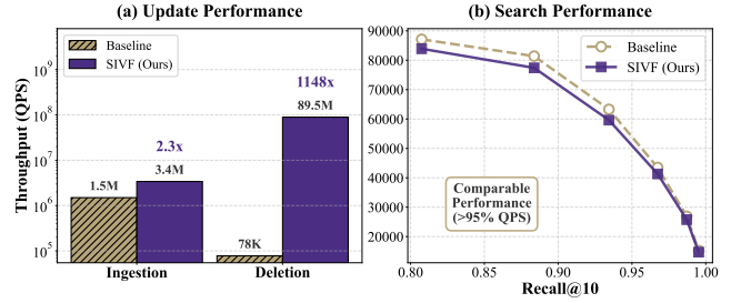
Figure 13: High-dimensional DINO10B dataset on 10 GPUs.
