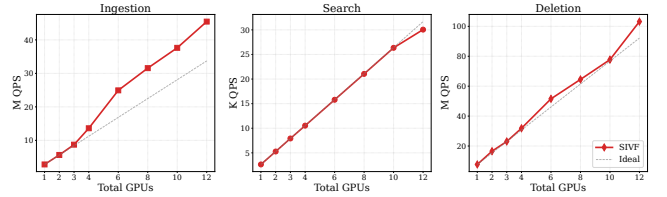
Figure 13: Scalability across a 4-node cluster of 12 GPUs.
