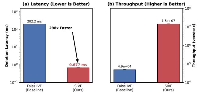
Figure 4: Performance comparison of vector deletion between Faiss IVF (Baseline) and SIVF.
