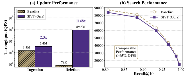
Figure 13: End-to-end performance on the high-dimensional DINO dataset (1024 dimensions) on a 10-GPU cluster.
