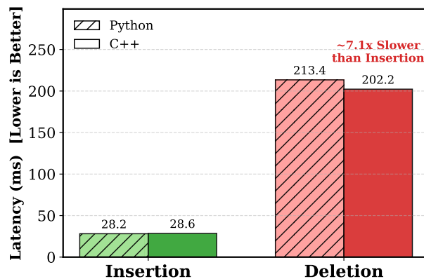
High Deletion Overhead: Python vs. C++
