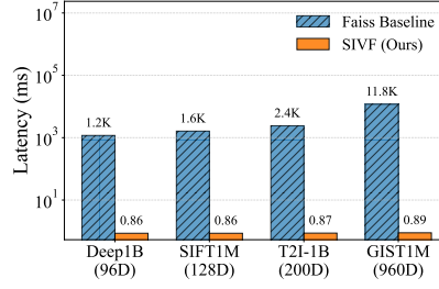
Figure 8: Deletion latency.
