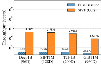
Figure 7: Ingestion throughput.
