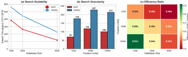
Figure 3: Microbenchmark performance of vector search.
