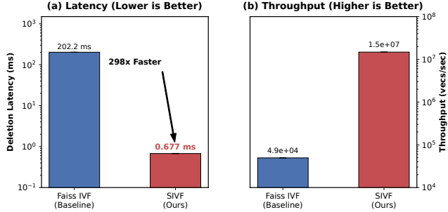
Figure 4: Microbenchmark performance of vector deletion.
