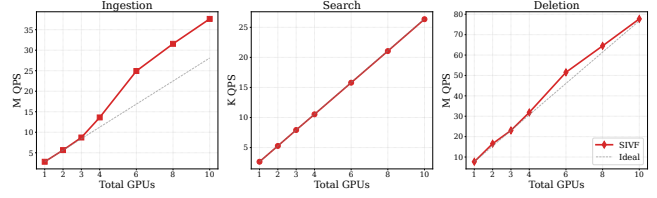
Figure 13: Scalability of SIVF core operations across a three node cluster with up to 10 GPUs.
