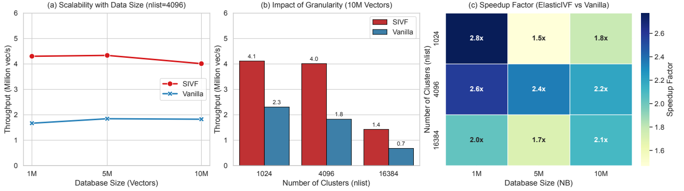
Figure 2: Performance evaluation of vector ingestion. (a) Scalability: Throughput remains stable around 4.0–4.3 million vec/s as dataset size increases ( n_{list} = 4096 ). (b) Granularity Impact: While both systems slow down at finer granularities ( n_{list} = 16384 ), ElasticIVF remains significantly faster than the baseline. (c) Speedup: A heatmap showing the relative speedup of ElasticIVF over Vanilla Faiss, consistently ranging between 1.5 \times and 2.8 \times .
