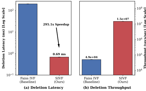
Figure 4: Performance comparison of vector deletion between Faiss IVF (Baseline) and SIVF. (a) shows the deletion latency in milliseconds on a log scale, where SIVF achieves a 295.1x speedup. (b) shows the deletion throughput in vectors per second on a log scale.
