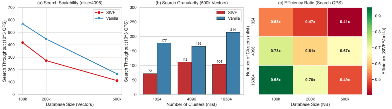
Figure 3: Performance evaluation of vector search. (a) Search Scalability: Both systems exhibit similar throughput degradation patterns as the database size grows from 100k to 500k. (b) Search Granularity: Finer clustering (higher n_{list} ) improves QPS by reducing the search space per probe. (c) Efficiency Ratio: Heatmap showing SIVF’s query throughput relative to Vanilla Faiss across different configurations.
