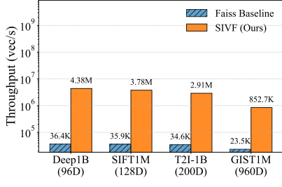
Figure 5: Ingestion throughput.
