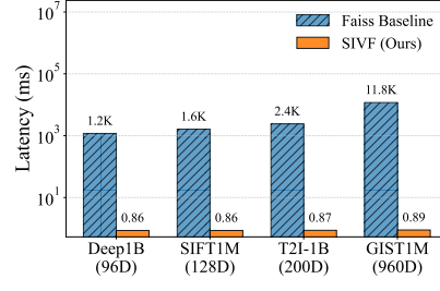
Figure 6: Deletion latency.
