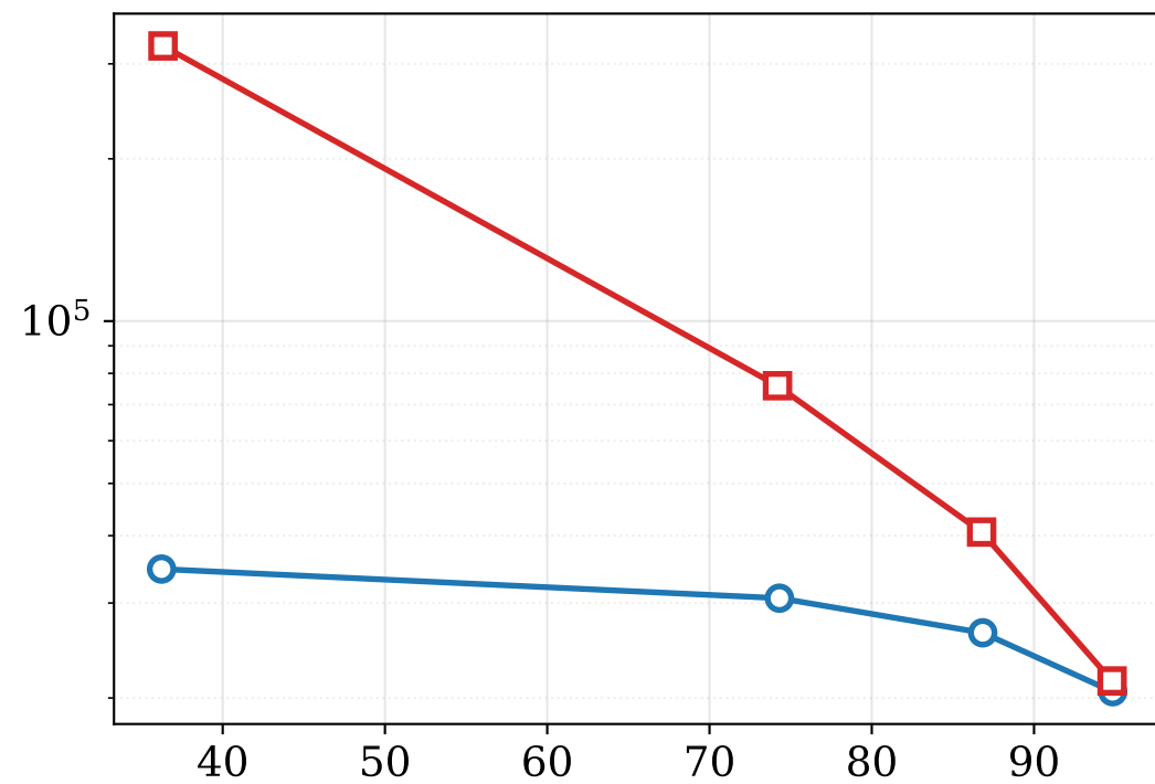
SIFT1M (128D)
