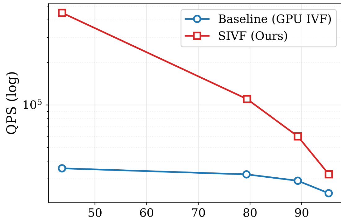
Deep1B (96D)
