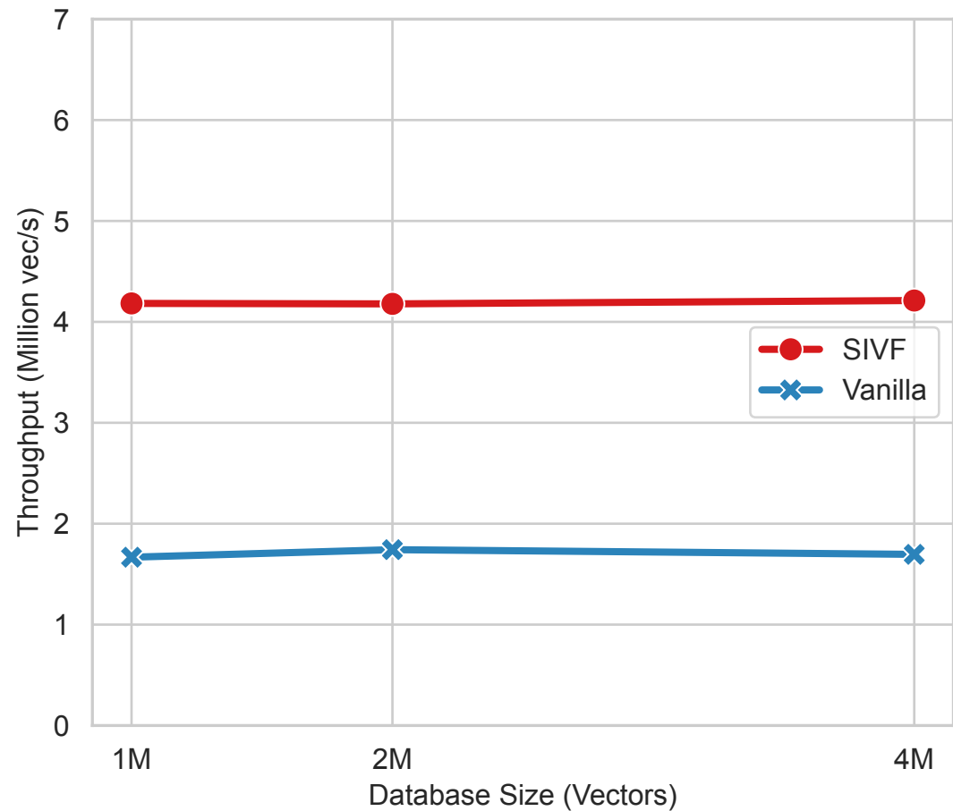
(a) Scalability with Data Size (nlist=4096)
