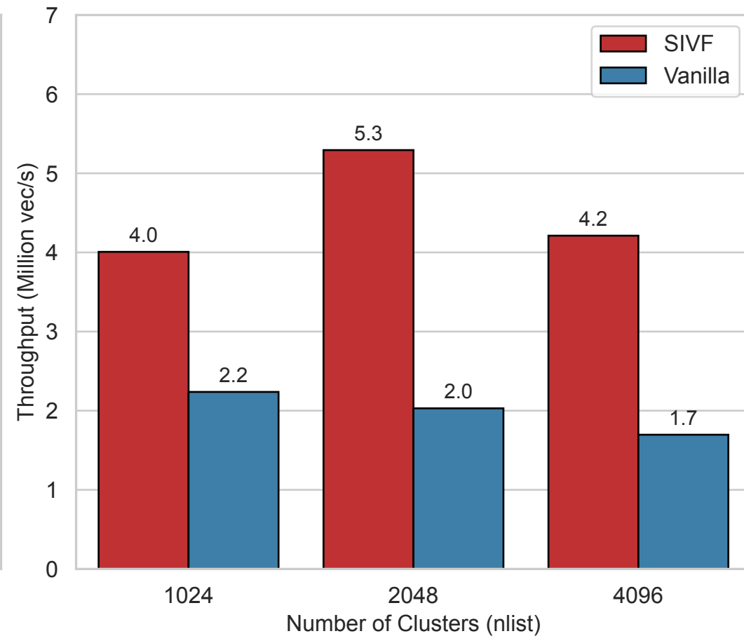
(b) Impact of Granularity (4M Vectors)
