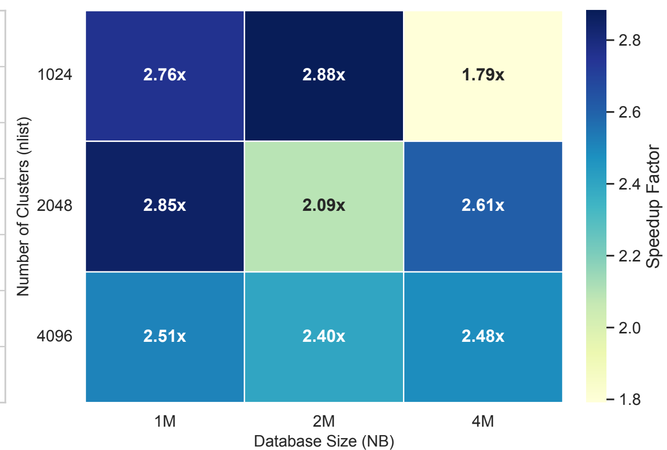
(c) Speedup Factor (ElasticIVF vs Vanilla)
