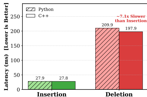
High Deletion Overhead: Python vs. C++
