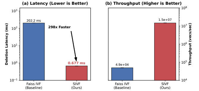
Figure 4: Performance comparison of vector deletion between Faiss IVF (Baseline) and SIVF. (a) Deletion latency (log scale), where SIVF achieves a 298.5\times reduction compared to the baseline. (b) Deletion throughput (log scale), demonstrating SIVF’s capacity to sustain over 14 million deletions per second.
