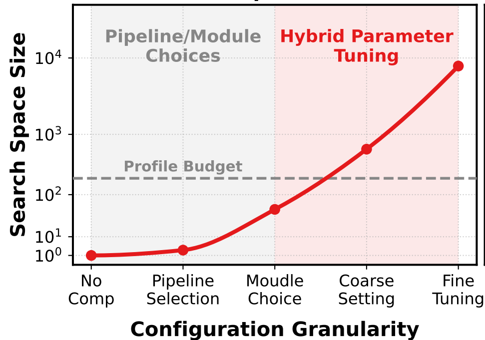
Search Space Growth
