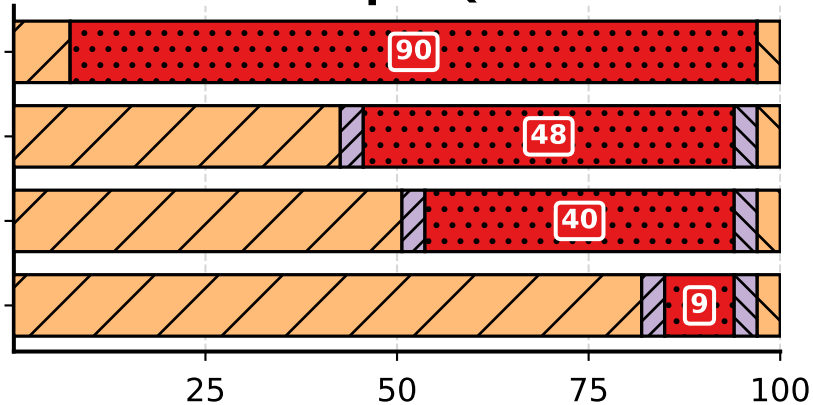
HotpotQA
