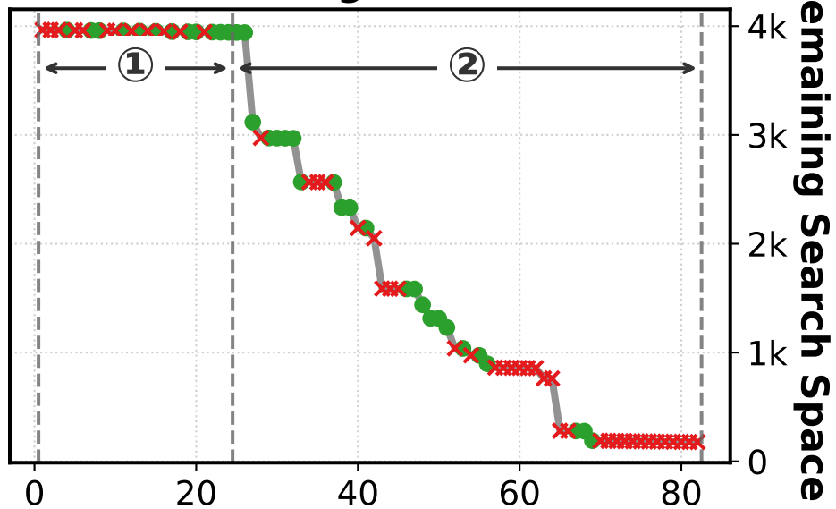
Pruning Process
