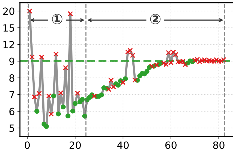
Prediction Process
