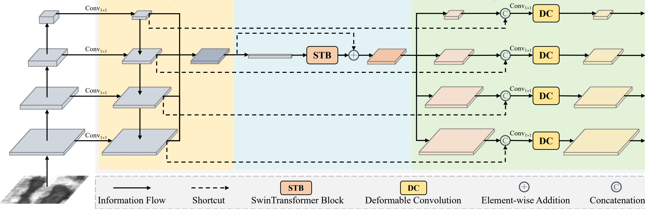
(a) Feature Aggregation
