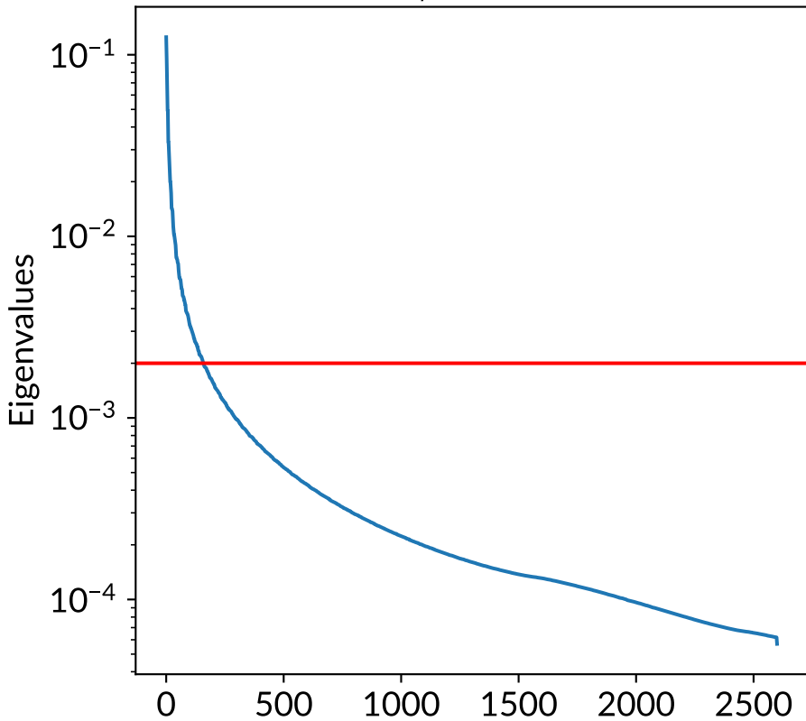
Eigenvalues of \Gamma_{pr} for bi-Laplacian prior
