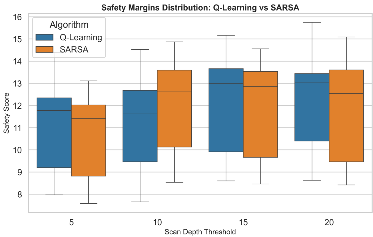
Figure 1 — Box Plot: Safety Margins per Scan Depth (Q-Learning vs SARSA)
