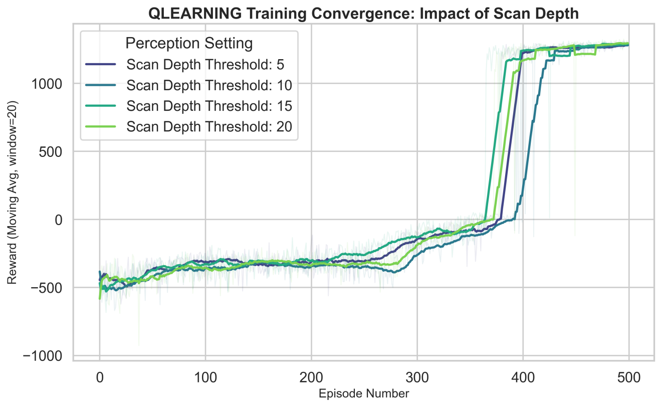
Figure 3 — Q-Learning: Reward Convergence across Scan Depths
