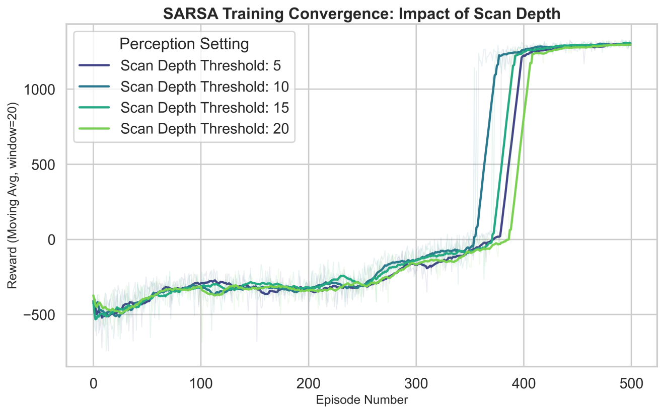
Figure 4 — SARSA: Reward Convergence across Scan Depths
