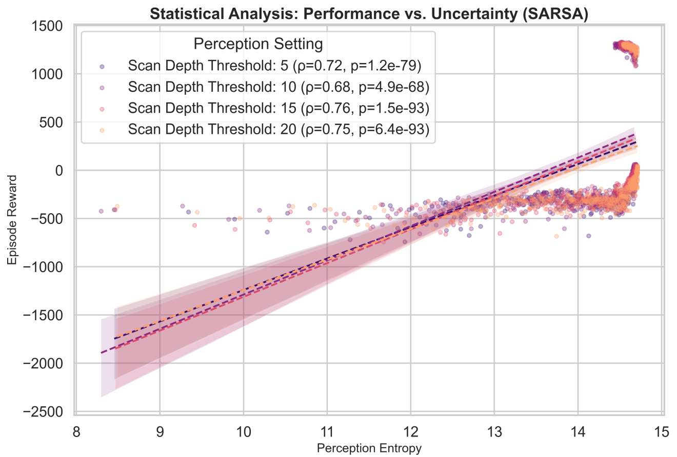
Figure 6 — SARSA: Episode Reward vs Perception Entropy (Spearman \rho )
