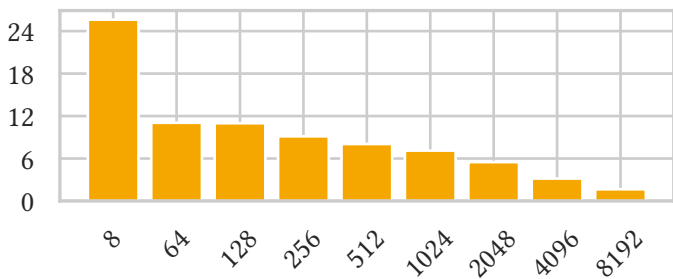
Valkey (sync)
