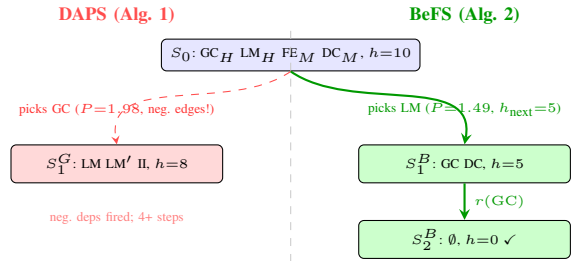
Fig. 2. DAPS vs. BeFS ordering trace.
