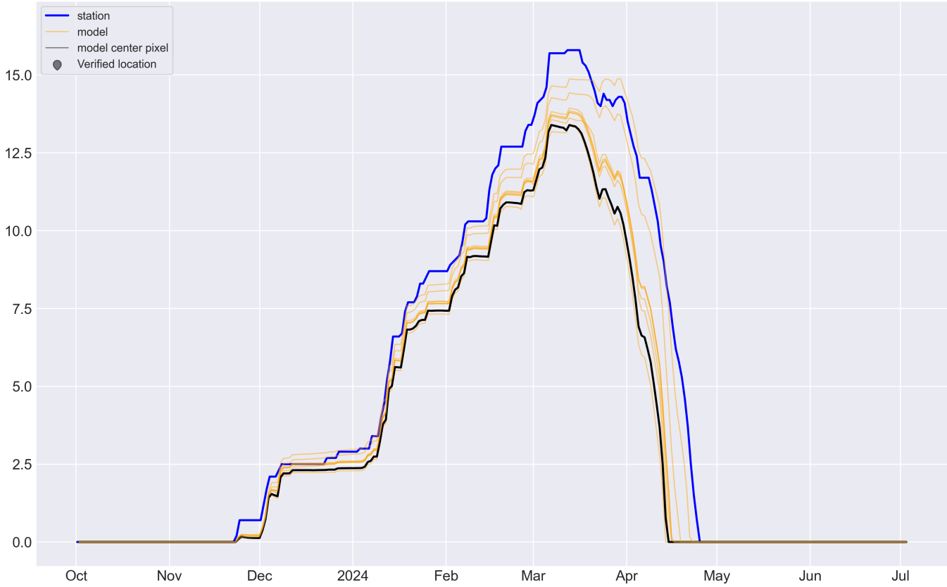
Fig.3 Comparison of modeled and measured Snow Water Equivalent [in.]. Comparisons of model pixels to measured station data are performed with the 9 nearest model pixels to give a more spatially complete view of model behavior.
