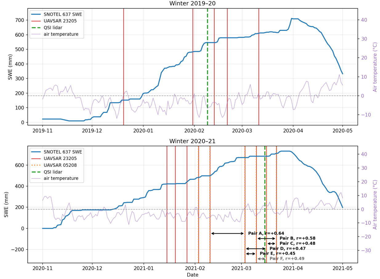
Mores Creek Summit SNOTEL SWE and air temperature, with UAVSAR flights, QSI lidar, and the selected InSAR pairs
