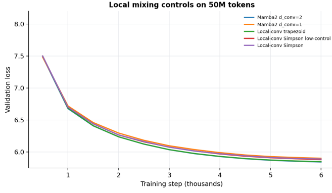
Fig. 8. Local-mixing controls. Adding Mamba2-style local mixing narrows the gap for Simpson, but local-conv trapezoid is still better at this budget.
