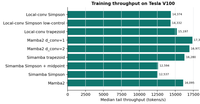
Fig. 9. Median tail training throughput on the V100, computed from the last 100 logged W&B points for each run.
