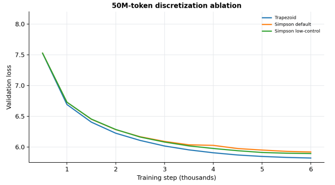
Fig. 7. 50M-token discretization ablation. The low-control initialization improves Simpson, but the matched trapezoid update remains ahead.
