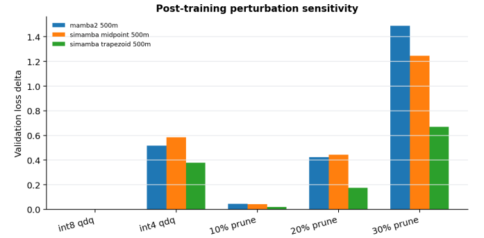
Fig. 12. Validation loss delta after post-training perturbations. Int8 row-wise quantize-dequantize is nearly lossless; int4 and larger pruning ratios require finetuning or better kernels.
