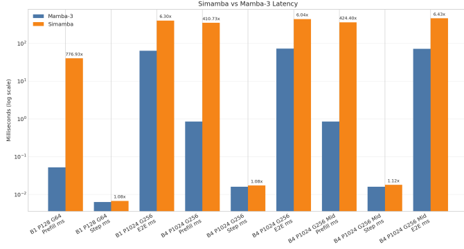
Fig. 10. Repository SISO benchmark latency. Simamba decode overhead is small, but the prefill implementation is not competitive without fused-kernel work.
