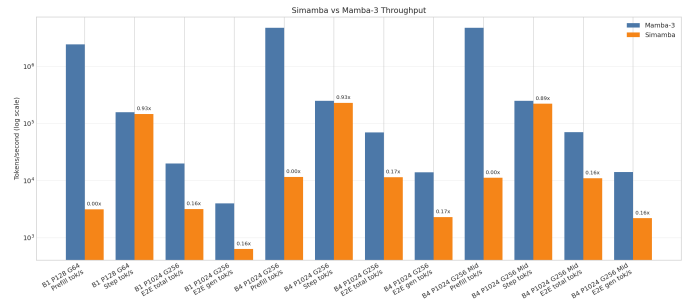
Fig. 10. Repository SISO benchmark throughput. The current prefill gap is a systems bottleneck independent of validation loss.
