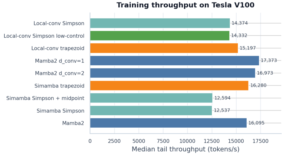
Fig. 10. Median tail training throughput on the V100, computed from the last 100 logged W&B points for each run.
