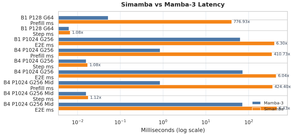
Fig. 11. Repository SISO benchmark latency. Simamba decode overhead is small, but the prefill implementation is not competitive without fused-kernel work.
