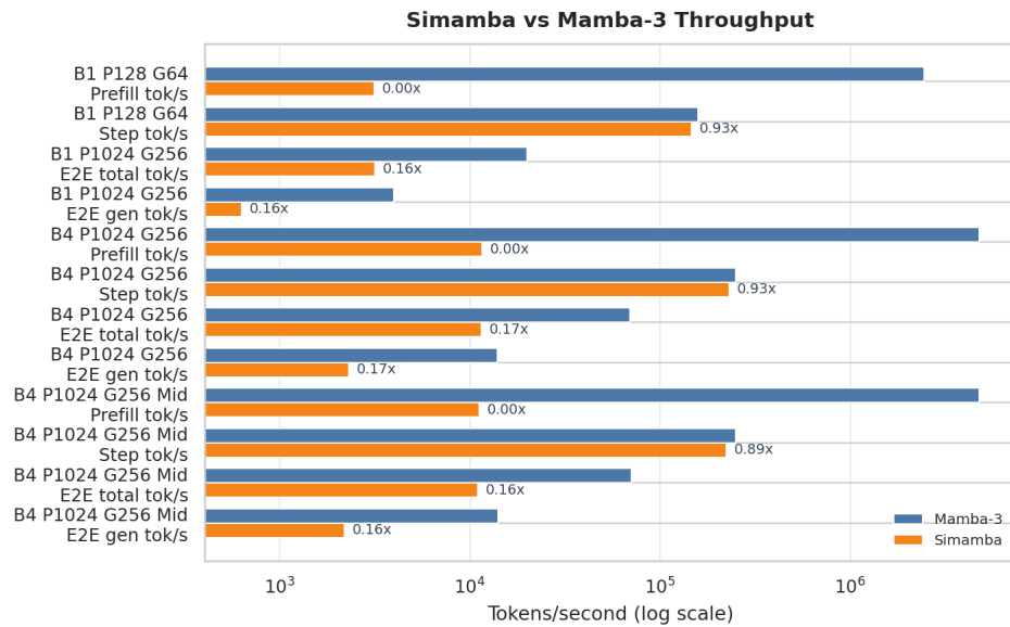
Fig. 12. Repository SISO benchmark throughput. The current prefill gap is a systems bottleneck independent of validation loss.
