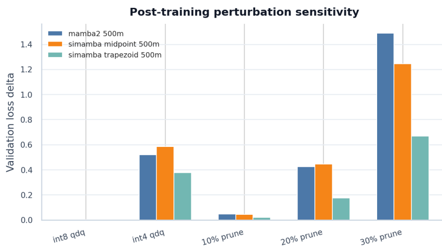
Fig. 15. Validation loss delta after post-training perturbations. Int8 row-wise quantize-dequantize is nearly lossless; int4 and larger pruning ratios require finetuning or better kernels.
