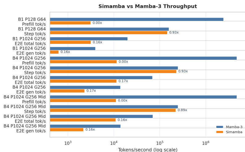
Fig. 10: Repository SISO benchmark throughput. The current prefill gap is a systems bottleneck independent of validation loss.
