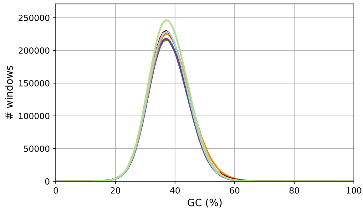
GC content
