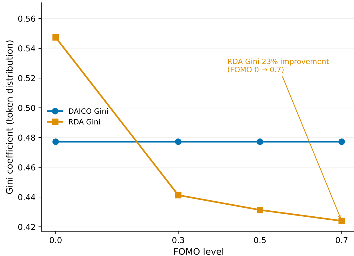
small_project (Solana-scale)
