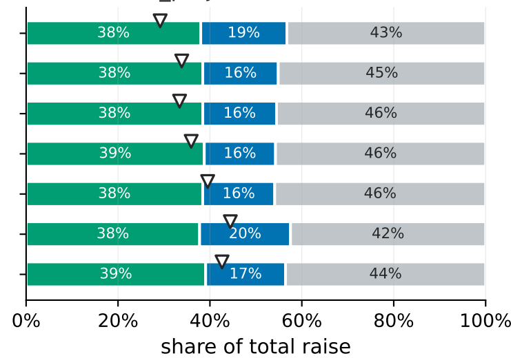
small_project (Solana-scale)
