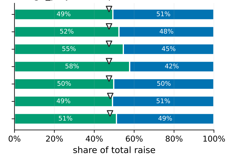
large_project (Casper/Mina/Flow-scale)
