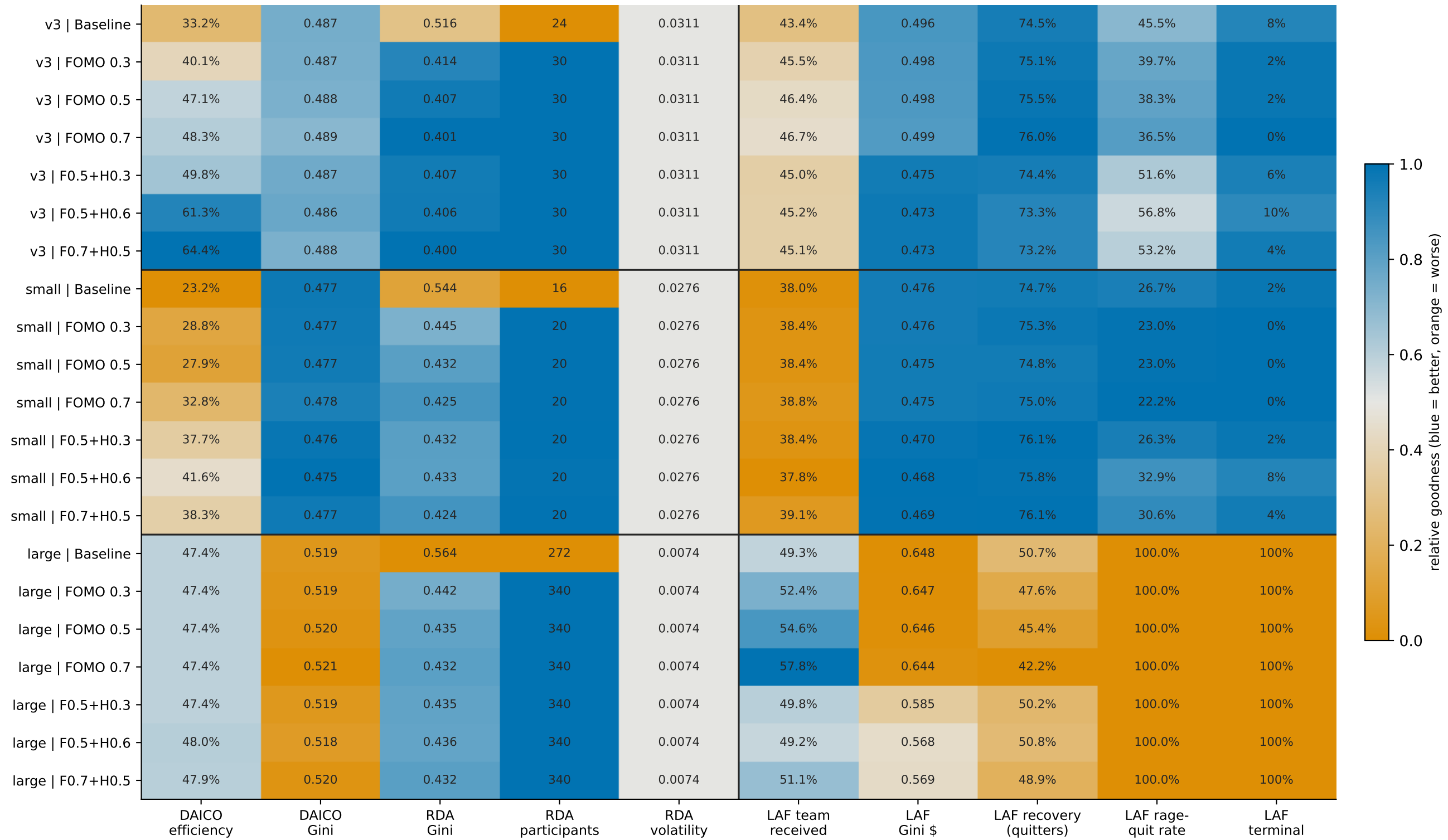
Metric comparison v5.0: 7 scenarios x 3 profiles, DAICO / RDA (left) and LAF (right) participants and volatility coloured within profile; all other columns coloured globally
