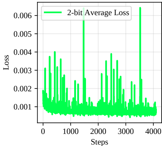
2-bit Quantization Training
