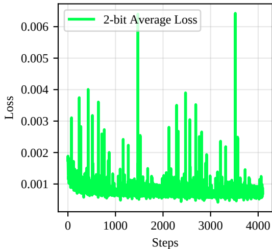
2-bit Quantization Training
