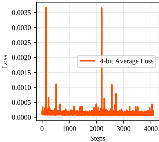
4-bit Quantization Training
